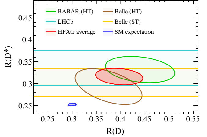
Figure 6. \mathcal{R}_D and \mathcal{R}_{D^*} measurements: Results from BABAR [28], Belle [34, 35], and LHCb [36], their values and 1\text{-}\sigma contours. The average calculated by the Heavy Flavor Averaging Group [37] is compared to SM predictions [19, 20, 21]. ST and HT refer to the measurements with semileptonic and hadronic tags, respectively.
