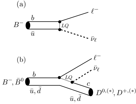
Figure 7. Diagrams for non-SM decay processes: (a) B^- \rightarrow \ell^- \bar{\nu}_\ell with a purely leptonic final state and (b) \bar{B} \rightarrow D^{(*)} \ell^- \bar{\nu}_\ell , involving a charm meson and lepton pair and mediated by a spin-0 lepto-quark (LQ).
